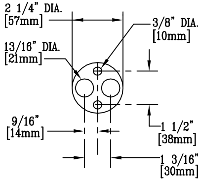
SHANK WASHER DETAIL
