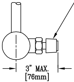
SIDE VIEW - 3"=1'
