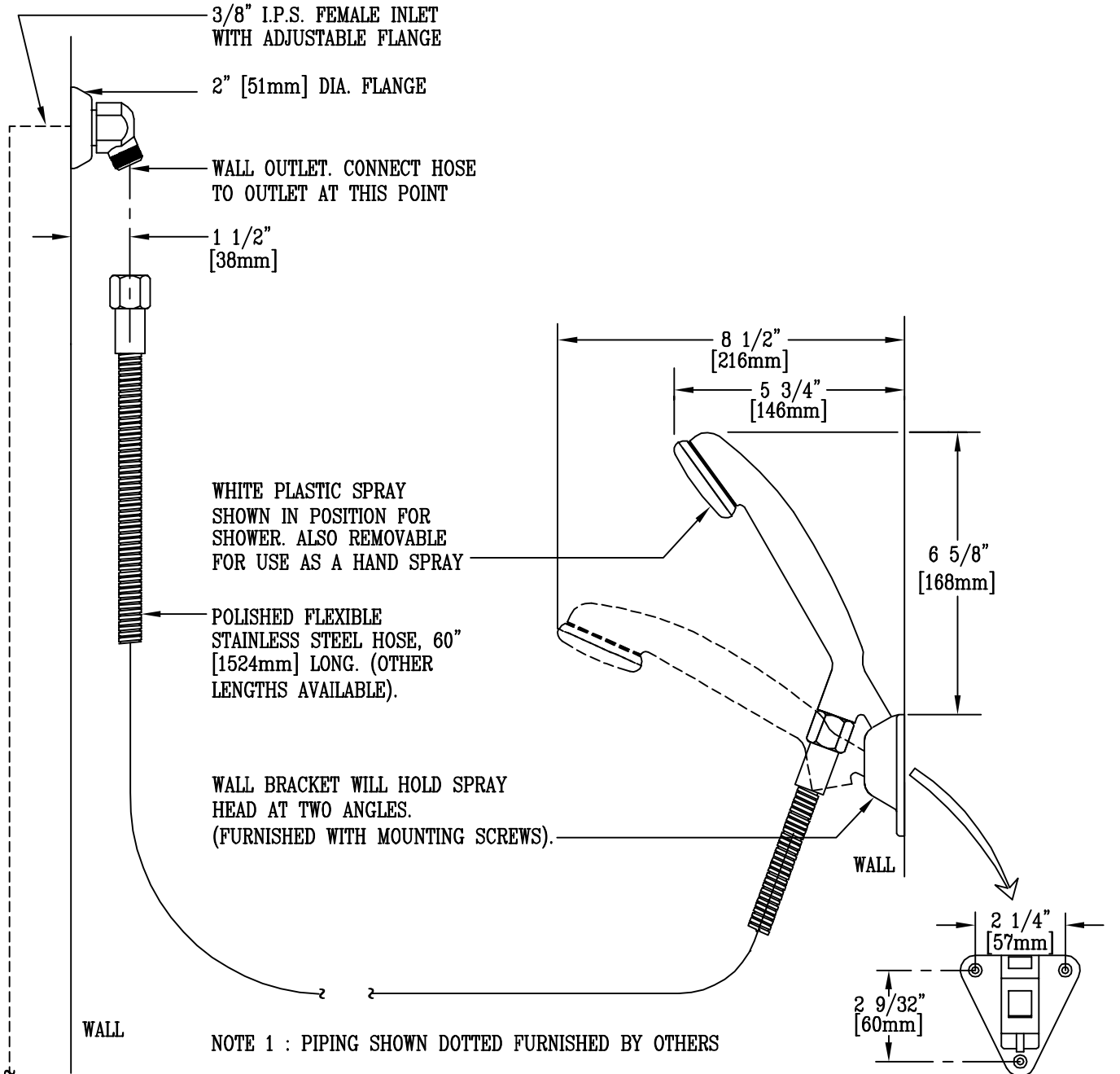
WALL BRACKET MOUNTING DETAIL
