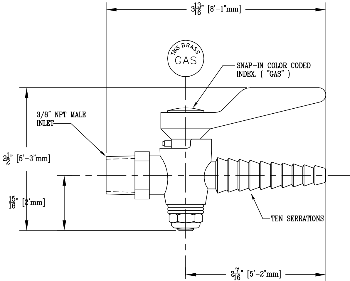
AGA AND CGA APPROVED GAS COCK WITH INTEGRAL CHECK
