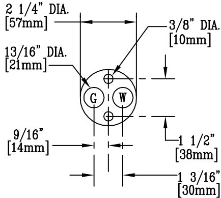
SHANK WASHER DETAIL
