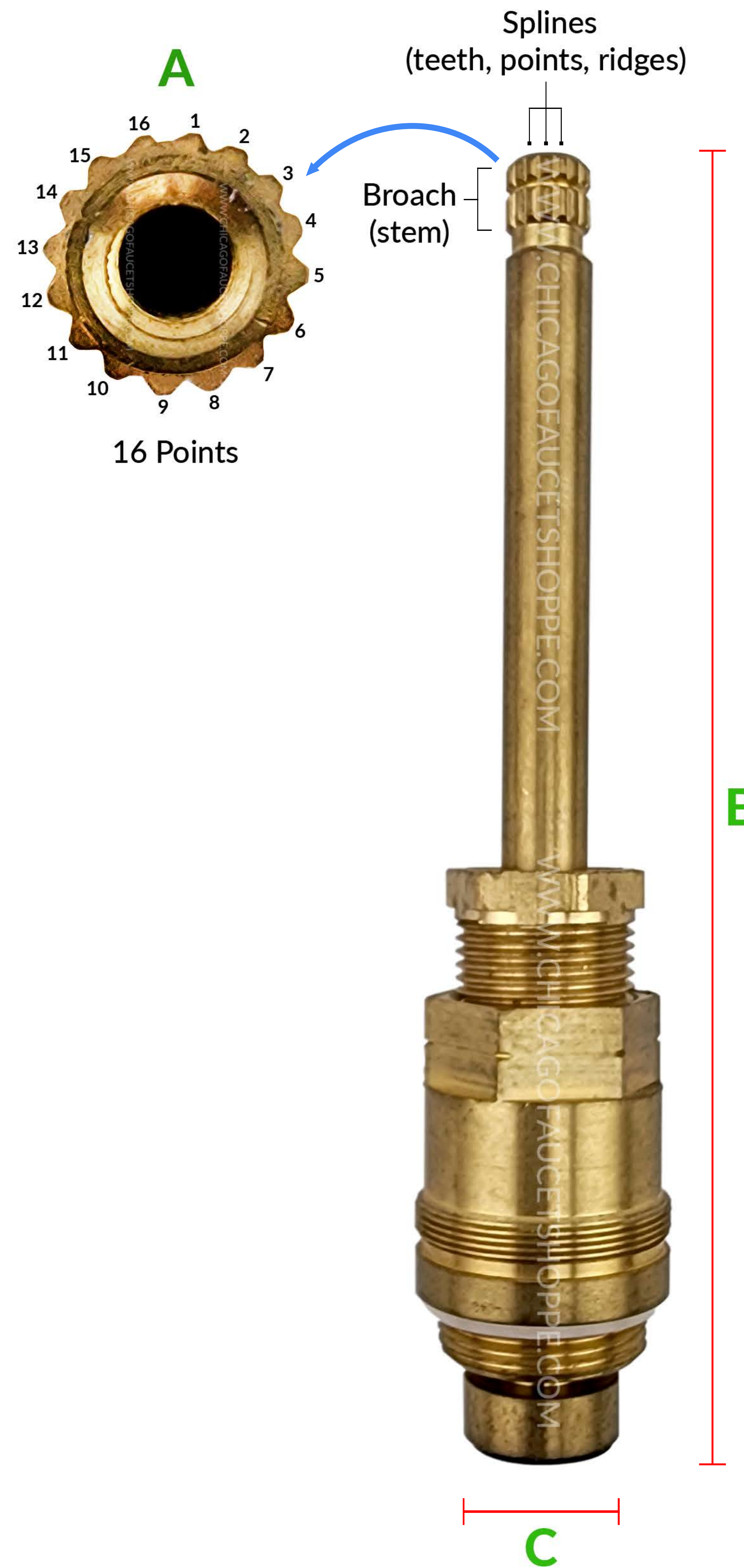
Compression Cartridge
