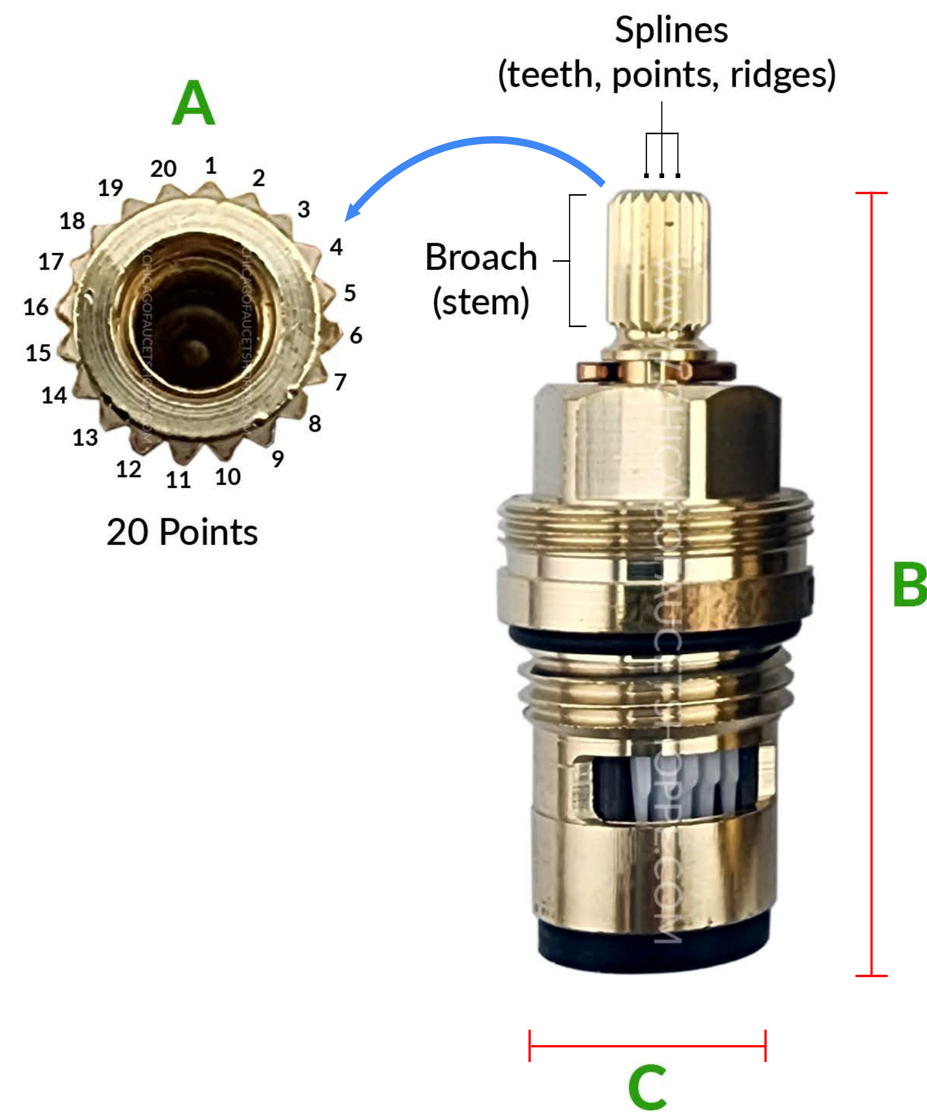
Ceramic Cartridge
